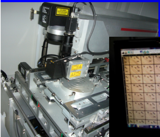
Laser/Inkjet Marking Machine
